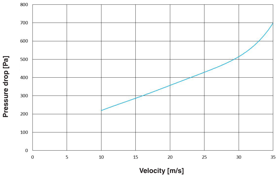
CARZ-NS 160 - 250 mm: Static Pressure
